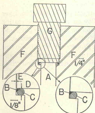
FIG. 1. Cross section of the high-pressure closure plug with armored O-ring seals. The inserts show the armor configuration before and after initial application of pressure to the system. A, the high-pressure region; B, machine steel armor ring; C, O-ring 7274 AN123872; D, O-ring squeeze; E, extrusion gap; F, bomb walls; G, closure plug.
