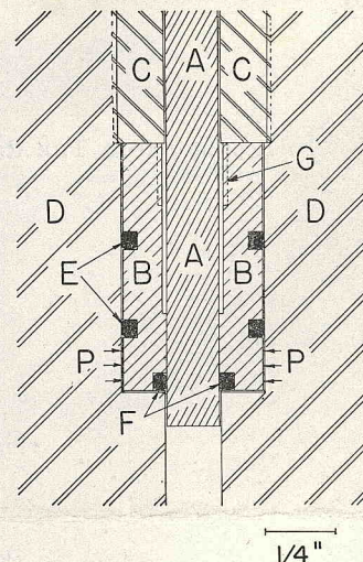
FIG. 3. Cross section of the high-pressure pump piston seal. A, reciprocating pump piston; B, phosphor bronze seal body; C, packing gland nut; D, body of pump; E, O-rings sealing outside of seal body, AN6227B-7; F, O-ring sealing between piston and inside of seal body, AN6227B-3; G, threaded portion to enable extraction of seal body; P, P indicates the re-entrant region of the seal body in which the seal is exposed to pump pressure on its outside but not on its inside surface.
