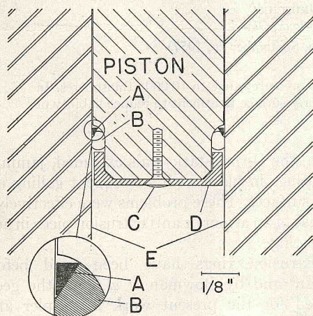
FIG. 2. Cross section of the high-pressure intensifier seal. The insert shows an enlarged cross section of the phosphor bronze armor ring. A, armor ring; B, O-ring AMS 7274 AN123861; C, 5-40 machine screw; D, filler piece to hold O-ring and armor in place during installation; E, walls of high-pressure cylinder.
